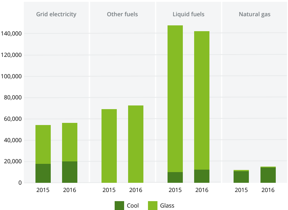
Total MWh of energy consumption per source
